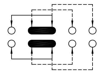
SCHEMATIC (SHORTING)
